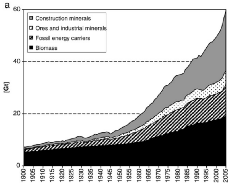
Figure 1: Materials use (DMC = DE) by material types in the period 1900 to 2005: total materials use in Giga tons (Gt) per year (Krausmann et al. 2009, 4)
